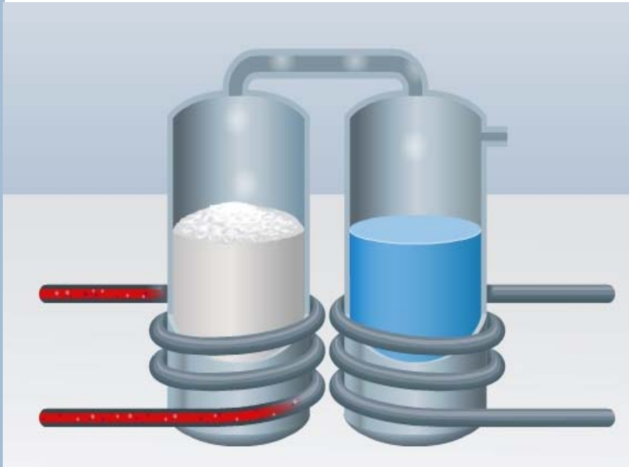
LiCl-Water Solution Pure Water
