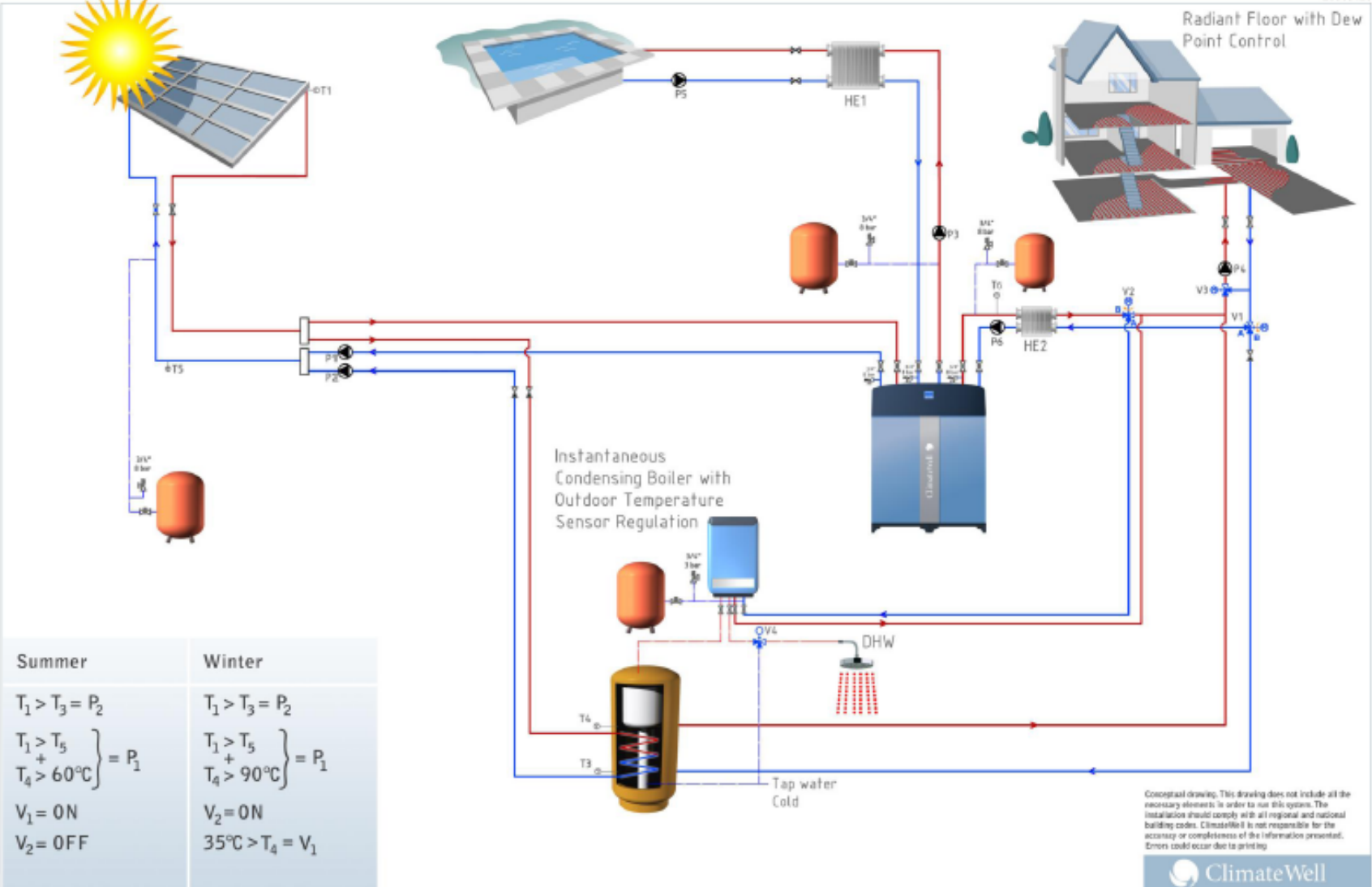
ClimateWell's Recommended Solar System Single Family 2
